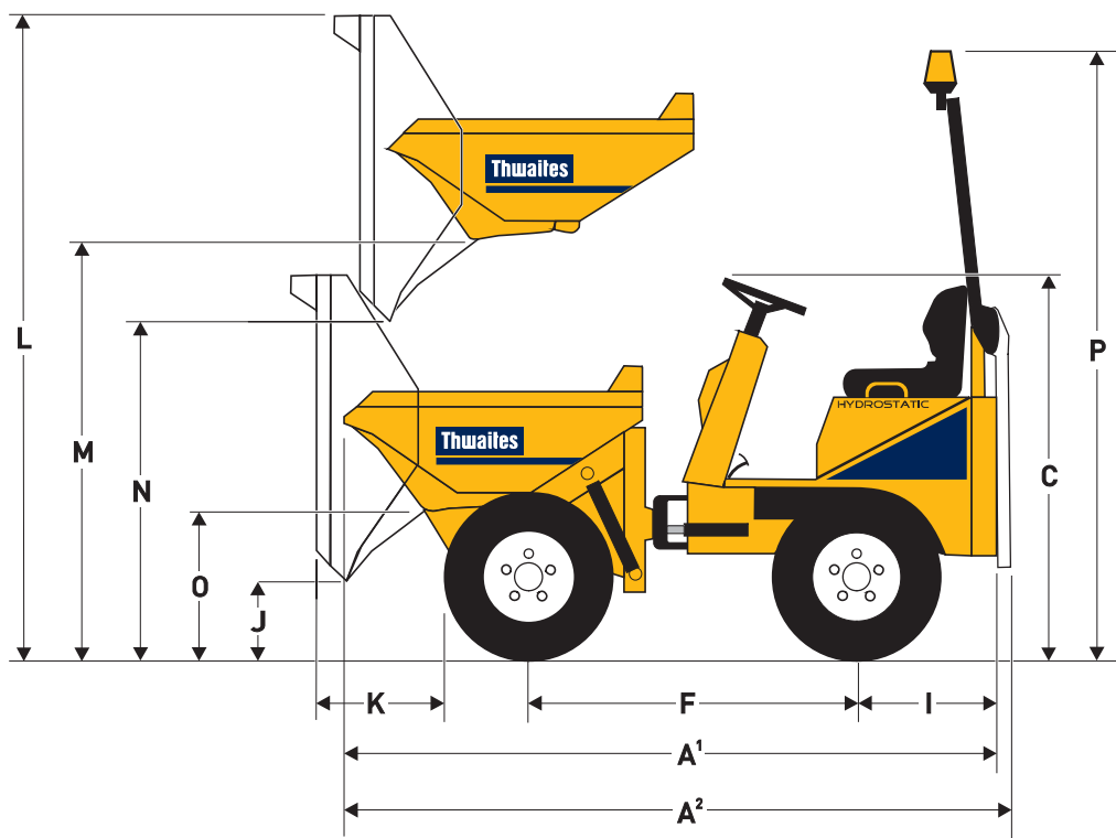
Dimensions (mm)
